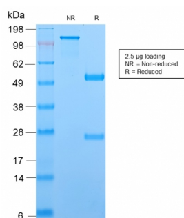
SDS-PAGE Analysis of Purified TCL1 Recombinant Rabbit Monoclonal Antibody (TCL1/2747R). Confirmation of Purity and Integrity of Antibody.
