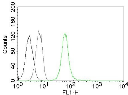
Flow Cytometry of human Vimentin on Jurkat cells. Black: cells alone; Grey: Isotype Control; Green: AF488-labeled Vimentin Mouse Monoclonal Antibody (VM452).
