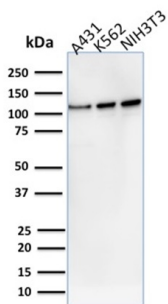
Western blot analysis of human A431, K562 and NIH3T3 cell lysates using Vinculin Mouse Monoclonal Antibody (VCL/2575).
