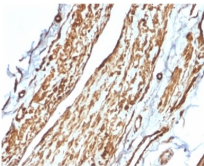
Formalin-fixed, paraffin-embedded human testicular carcinoma stained with Vinculin Mouse Monoclonal Antibody (VCL/2575) at 2ug/ml.
