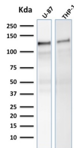
Western blot analysis of human U-87 and THP-1 cell lysates using Vinculin Mouse Monoclonal Antibody (VCL/2575).
