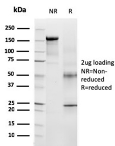
SDS-PAGE Analysis of Purified TYRP1-Monospecific Mouse Monoclonal Antibody (TYRP1/3283). Confirmation of Purity and Integrity of Antibody.
