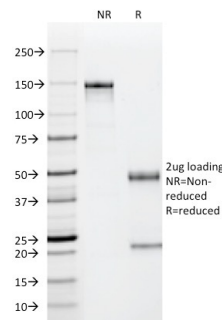
SDS-PAGE Analysis of Purified p53 Mouse Monoclonal Antibody (PAb122). Confirmation of Purity and Integrity of Antibody.
