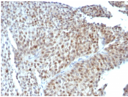
Formalin-fixed, paraffin-embedded human Bladder Carcinoma stained with p53 Monoclonal Antibody (SPM589).
