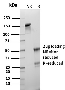
SDS-PAGE Analysis of Purified Cellular tumor antigen p53 Mouse Monoclonal Antibody (SPM589). Confirmation of Purity and Integrity of Antibody.
