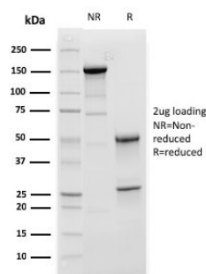
SDS-PAGE Analysis of Purified C1QA Mouse Monoclonal Antibody (C1QA/2952). Confirmation of Purity and Integrity of Antibody.
