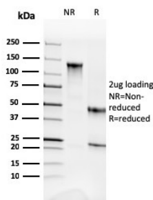
SDS-PAGE Analysis of Purified Fodrin Mouse Monoclonal Antibody (SPTAN1/3352). Confirmation of Purity and Integrity of Antibody.
