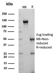
SDS-PAGE Analysis of Purified SOD1 Mouse Monoclonal Antibody (SOD1/3924). Confirmation of Purity and Integrity of Antibody.
