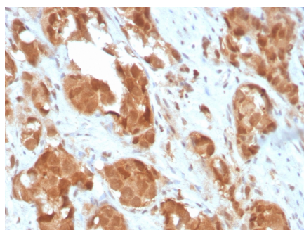
Formalin-fixed, paraffin-embedded human prostate stained with Superoxide Dismutase 1 Mouse Monoclonal Antibody (SOD1/3924).
