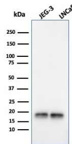
Western Blot Analysis of JEG-3 and LNCaP cell lysates using Superoxide Dismutase 1 Mouse Monoclonal Antibody (SOD1/3924).
