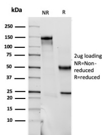
SDS-PAGE Analysis Purified S100B Mouse Monoclonal Antibody (SPM354). Confirmation of Purity and Integrity of Antibody.
