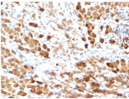
Formalin-fixed, paraffin-embedded human Melanoma stained with S100B Mouse Monoclonal Antibody (SPM354).
