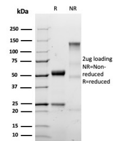
SDS-PAGE Analysis Purified S100A4 Recombinant Rabbit Monoclonal Antibody (S100A4/2750R). Confirmation of Purity and Integrity of Antibody.
