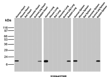
Western Blot Analysis of Heart, Lung and Spleen tissue lysates of different species using S100A4 Recombinant Rabbit Monoclonal Antibody (S100A4/2750R).
