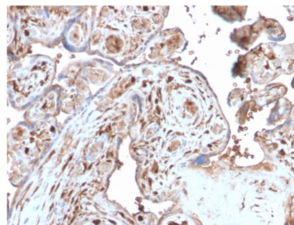
Formalin-fixed, paraffin-embedded human Placenta stained with S100A4 Recombinant Rabbit Monoclonal Antibody (S100A4/2750R).
