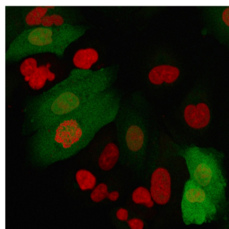
Immunofluorescence staining of A549 cells using S100A4 Recombinant Rabbit Monoclonal Antibody (S100A4/2750R) followed by goat anti-Mouse IgG-CF488 (green). Nuclei are stained with Reddot.
