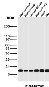
Western Blot Analysis of Human Heart, Human Lung, Human Spleen, Human Ovary, A549, and HeLa lysates using S100A4 Recombinant Rabbit Monoclonal Antibody (S100A4/2750R).
