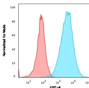
Flow Cytometric Analysis of A549 cells using S100A4 Recombinant Rabbit Monoclonal Antibody (S100A4/2750R) followed by goat anti-rabbit IgG-CF488 (Blue); Isotype Control (Red).
