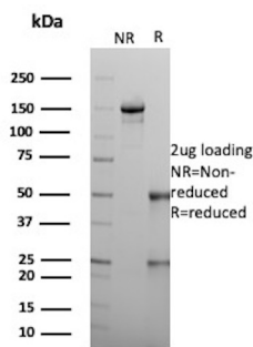
SDS-PAGE Analysis of Purified RBP4 Mouse Monoclonal Antibody (RBP4/4048). Confirmation of Purity and Integrity of Antibody.
