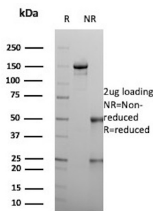
SDS-PAGE Analysis of Purified Retinol-binding protein 4 Mouse Monoclonal Antibody (RBP4/4048). Confirmation of Purity and Integrity of Antibody.
