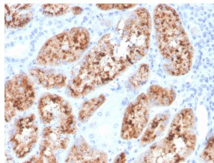
Formalin-fixed, paraffin-embedded human kidney stained with RBP4 Mouse Monoclonal Antibody (RBP4/4048).
