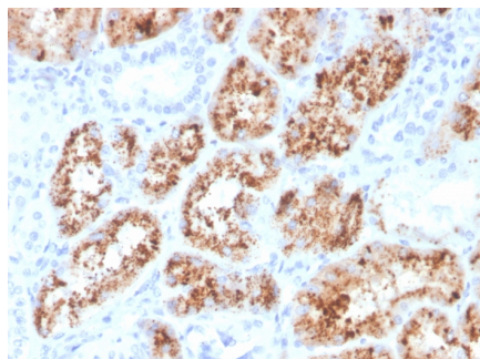
Formalin-fixed, paraffin-embedded human kidney stained with RBP4 Mouse Monoclonal Antibody (RBP4/4048).
