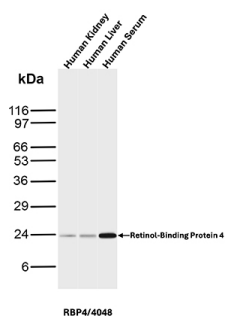
Western blot analysis of human kidney and liver tissue lysates and human serum samples using Retinol-Binding Protein 4 Recombinant Mouse Monoclonal Antibody (RBP4/4048).
