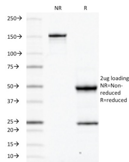
SDS-PAGE Analysis of Purified CD45RB Mouse Monoclonal Antibody (PD7/26). Confirmation of Purity and Integrity of Antibody.
