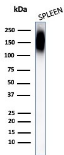
Western Blot Analysis of human Spleen tissue lysates using CD45RA Mouse Monoclonal Antibody (158-D3).
