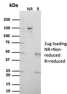
SDS-PAGE Analysis of Purified Receptor-type tyrosine-protein phosphatase C Mouse Monoclonal Antibody (PTPRC/1147). Confirmation of Purity and Integrity of Antibody.
