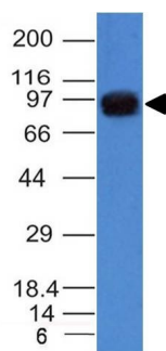
Western Blot of A549 cell lysate using UACA / Nucling Monoclonal Antibody (AE-5)
