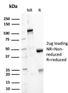
SDS-PAGE Analysis of Purified Stromelysin-1 Recombinant Rabbit Monoclonal Antibody (MMP3/1994R). Confirmation of Purity and Integrity of Antibody.
