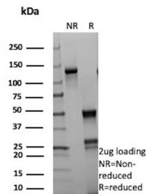
SDS-PAGE Analysis of Purified DNA mismatch repair protein Mlh1 Recombinant Mouse Monoclonal Antibody (rMLH1/6285). Confirmation of Purity and Integrity of Antibody.
