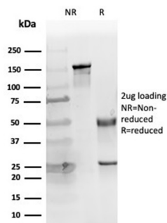
SDS-PAGE Analysis of Purified Cytokeratin 14 Mouse Monoclonal Antibody (KRT14/4127). Confirmation of Purity and Integrity of Antibody.
