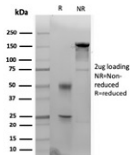
SDS-PAGE Analysis of Purified Cytokeratin 14 Mouse Monoclonal Antibody (KRT14/4133). Confirmation of Purity and Integrity of Antibody.
