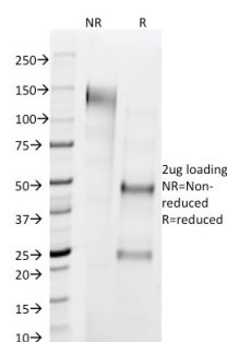
SDS-PAGE Analysis of Purified Cytokeratin 1 Mouse Monoclonal Antibody (LHK1). Confirmation of Integrity and Purity of Antibody.
