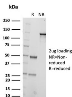
SDS-PAGE Analysis of Purified Integrin beta-3 Recombinant Rabbit Monoclonal Antibody (ITGB3/2166R). Confirmation of Purity and Integrity of Antibody.
