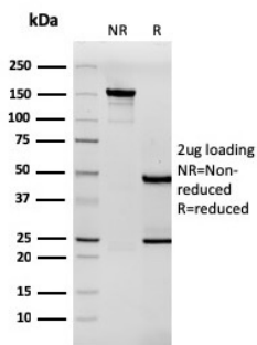
SDS-PAGE Analysis of Purified Tenascin C Mouse Recombinant Monoclonal Antibody (rTNC/3635). Confirmation of Purity and Integrity of Antibody.
