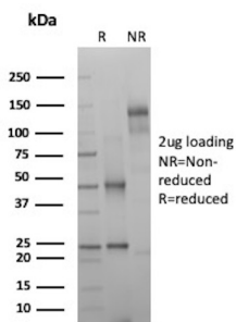
SDS-PAGE Analysis of Purified MHC I Mouse Monoclonal Antibody [SPM418]. Confirmation of Purity and Integrity of Antibody.
