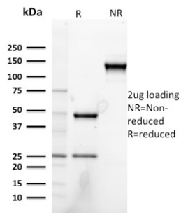
SDS-PAGE Analysis of Purified Heregulin-1 Mouse Monoclonal Antibody (NRG1/2752). Confirmation of Purity and Integrity of Antibody.
