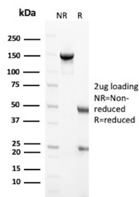
SDS-PAGE Analysis of Purified Somatotropin Recombinant Mouse Monoclonal Antibody (rGH/1450). Confirmation of Purity and Integrity of Antibody.
