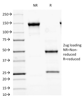
SDS-PAGE Analysis of Purified GAD2 (GAD65) Mouse Monoclonal Antibody (GAD2/2362). Confirmation of Purity and Integrity of Antibody.
