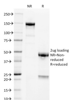
SDS-PAGE Analysis of Purified PLAP Mouse Monoclonal Antibody (GM022).
