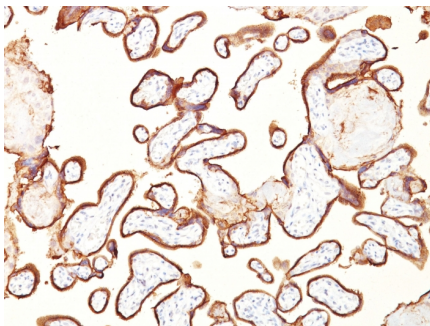
Formalin-fixed, paraffin-embedded human placenta stained with PLAP Mouse Monoclonal Antibody (GM022).
