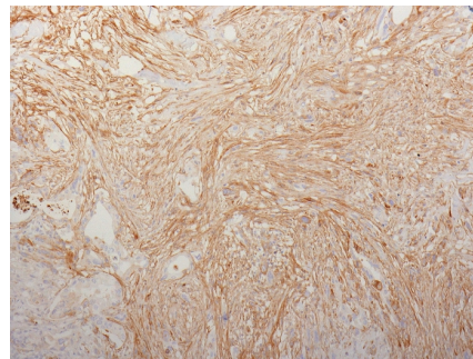
Formalin-fixed, paraffin-embedded human Pancreatic Adenocarcinoma stained with Fibronectin Monoclonal Antibody (HFN7.1).
