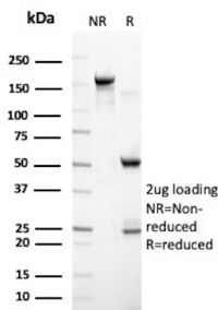
SDS-PAGE Analysis of Purified Fibronectin Mouse Monoclonal Antibody (HFN7.1). Confirmation of Purity and Integrity of Antibody.
