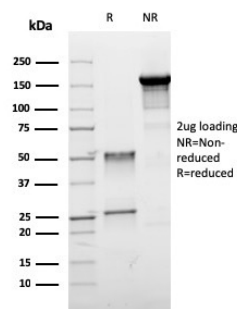
SDS-PAGE Analysis of Purified ER-beta Mouse Monoclonal Antibody (ESR2/3005). Confirmation of Purity and Integrity of Antibody.
