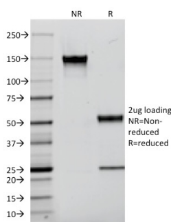
SDS-PAGE Analysis of Purified AIF1 / Iba1 Mouse Monoclonal Antibody (AIF1/2493). Confirmation of Integrity and Purity of Antibody.
