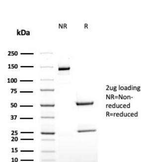
SDS-PAGE Analysis of Purified TAG-72 Recombinant Mouse Monoclonal Antibody (rB72.3). Confirmation of Purity and Integrity of Antibody.
