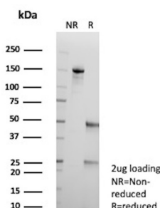
SDS-PAGE Analysis of Purified AKR1C1 Mouse Monoclonal Antibody (CPTC-AKR1C1-2). Confirmation of Purity and Integrity of Antibody.
