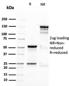
SDS-PAGE Analysis Purified Nestin Mouse Monoclonal Antibody (NES/2911). Confirmation of Purity and Integrity of Antibody.
