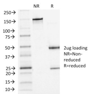
SDS-PAGE Analysis of Purified P-Cadherin Mouse Monoclonal Antibody (6A9). Confirmation of Integrity and Purity of Antibody.
